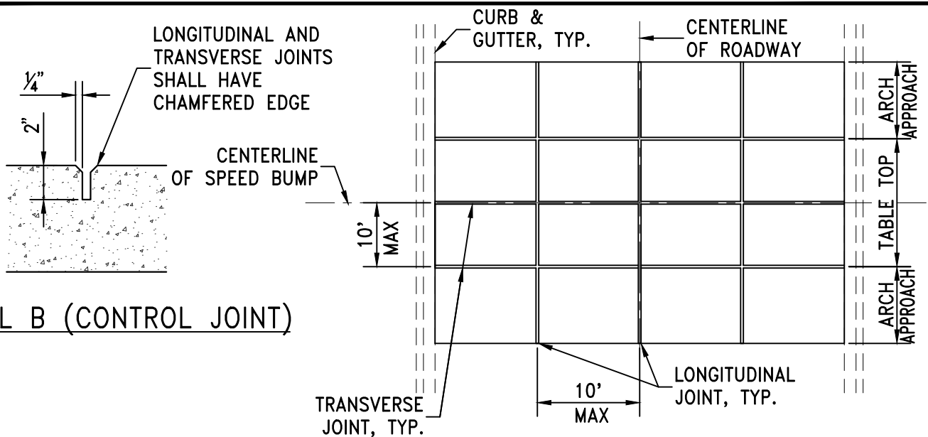
CONTROL JOINT PATTERN
